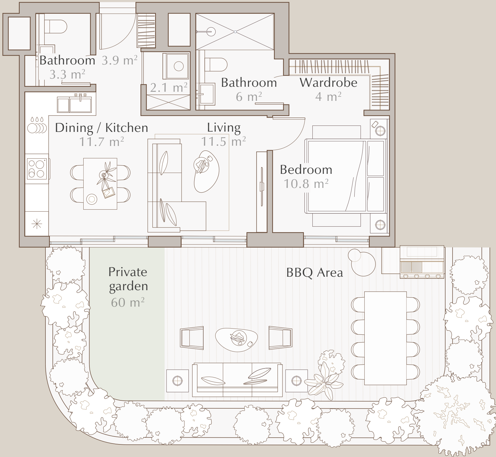
1 BEDROOM APARTMENT, TYPE A3G
